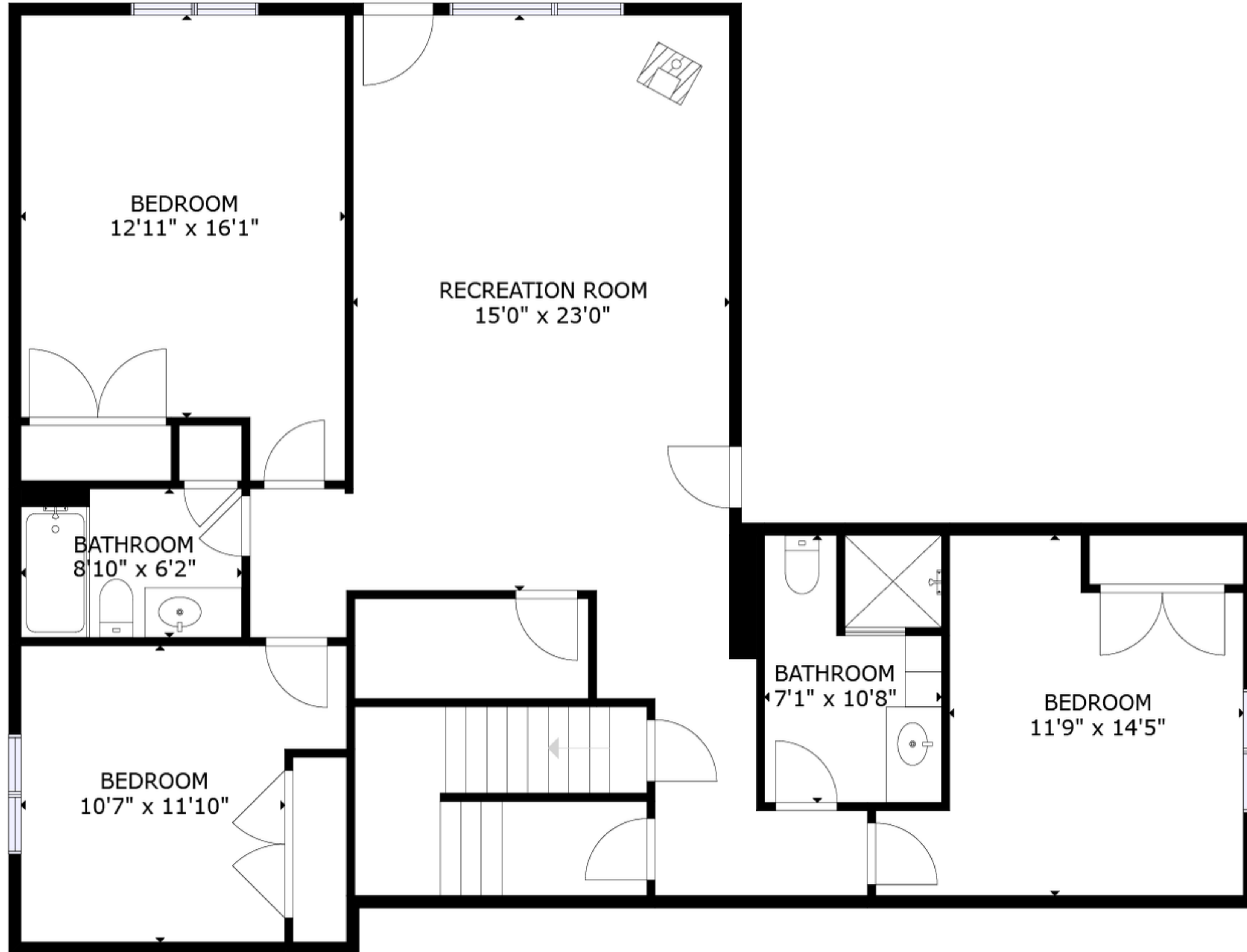
BASEMENT 1
